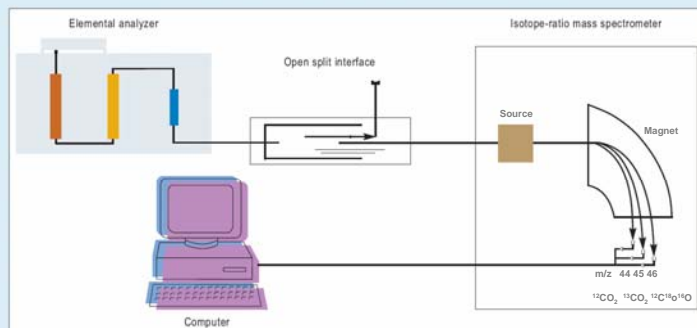
Schematic drawing of a Finnigan elemental analyzer/isotope-ratio mass spectrometer (EA/IRMS) 1
