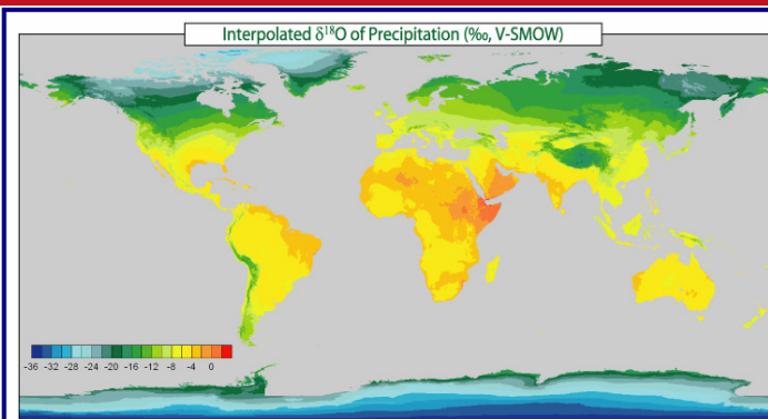
Figure 1: Diagram showing global variation of ^{18}\text{O} isotopic abundance in rain water [3].
