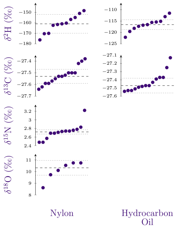
Results from FIRMS PT scheme Round 221. The lines represent the median of the results (dashed) plus or minus the robust standard deviation (dotted) following the exclusion of outliers.
